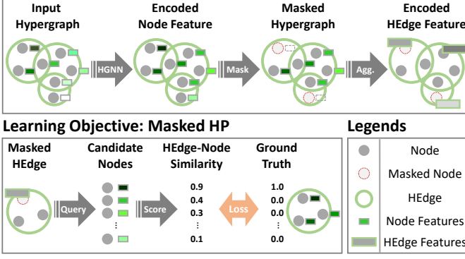
Fig. 5. The architecture and learning objective of MHP. HP stands for hyperedge prediction, and HEdge stands for hyperedge.
