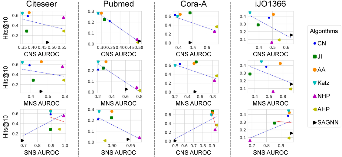
Fig. 3. “ Prediction is NOT classification. ” The relationship between classification performances (on the X-axis) and prediction performances (on the Y-axis) in HP. The correlations (depicted by blue dotted lines) are generally weak and mostly even negative. Moreover, all positive correlations are weak, and removing the single worst-performing method leads to negative correlations (depicted by red solid lines).
